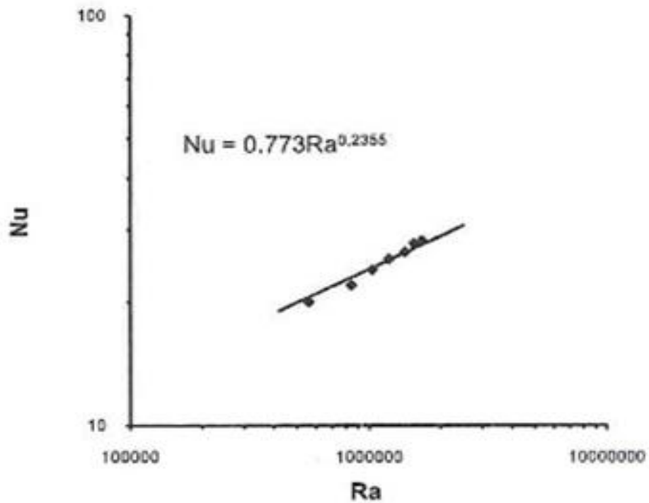
Figure (5):- The relationship between the Rayleighnumber and the average of Nusselt number at )m=0. 5(
