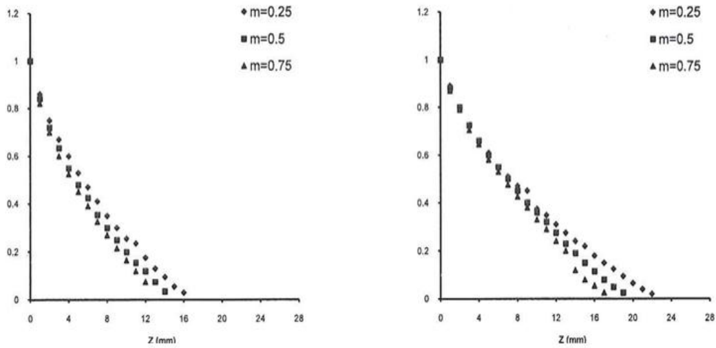
Figure (9):- Temperature distribution over the outer edge of the hollow surfaces at Ra=1033100.
