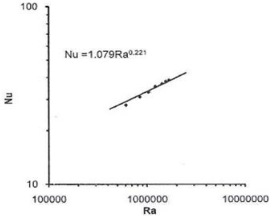
Figure (4):- The relationship between Rayleigh's number and the average of Nusselt number at )m=0.25(
