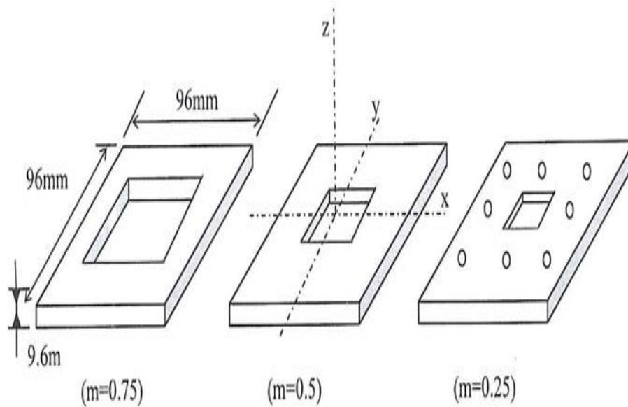
Figure (2):- Dimensions of the three aluminum sheets used with holes for thermocouples.
