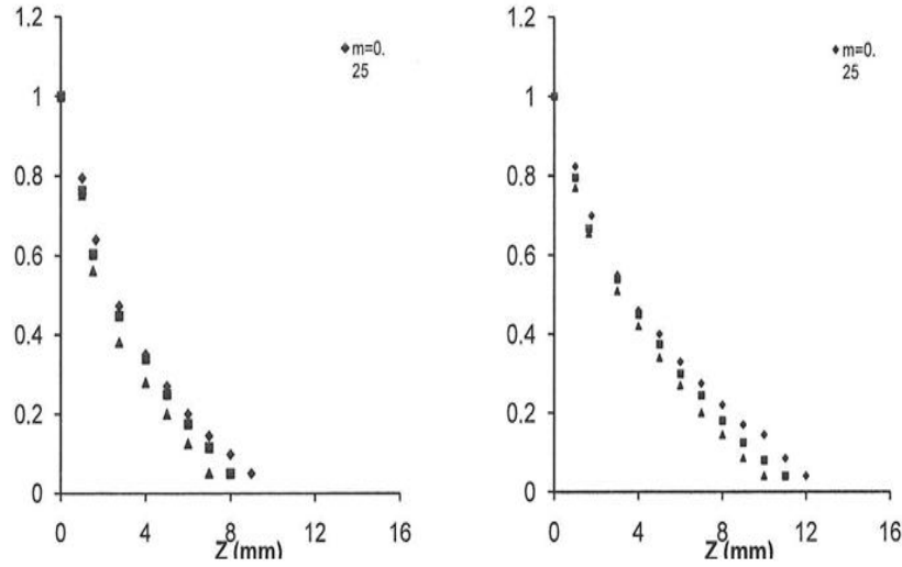
Figure (8):- Temperature distribution over the outer edge of the hollow surfaces at Ra=560000.
